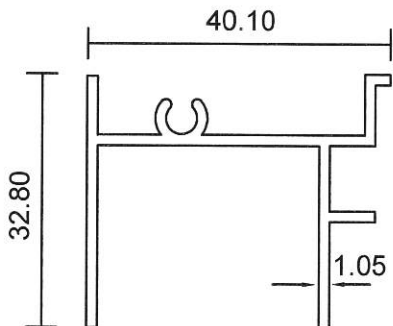
9352 0.381 Kg/m
