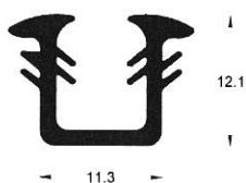
PSD Gasket 8mm Glass
