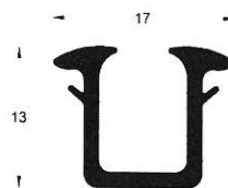
PSD Gasket 13.52mm Glass
