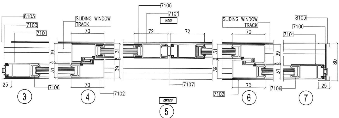
HORIZONTAL SECTION
