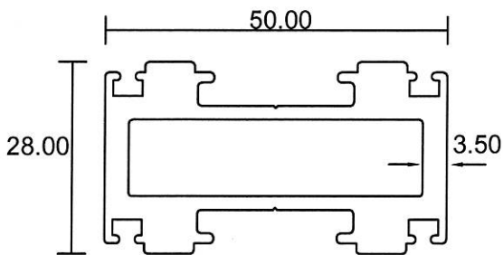
SLF-3513 1.494 Kg/m
