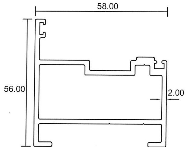
SLF-3503 1.297 Kg/m
