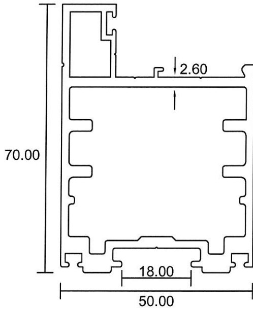
SLF-3511 1.900 Kg/m
