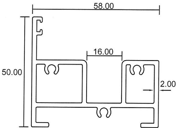
SLF-3502 1.325 Kg/m
