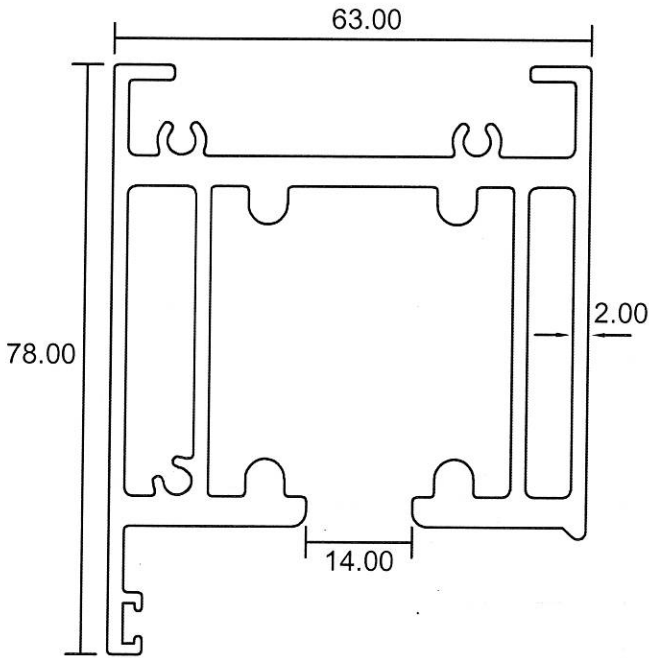
SLF-3501 2.778 Kg/m
