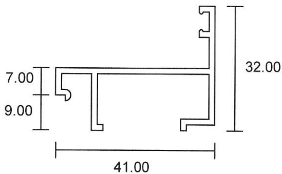
0422 0.313 Kg/m Casement Adaptor
