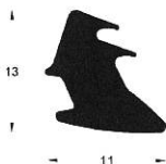
ESD Gasket Inner 13.52mm Glass
