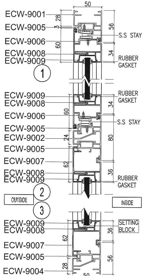
VERTICAL SECTION
