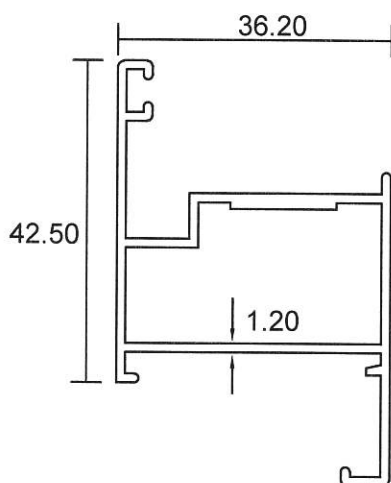
CW9103 0.606 Kg/m Casement Inner
