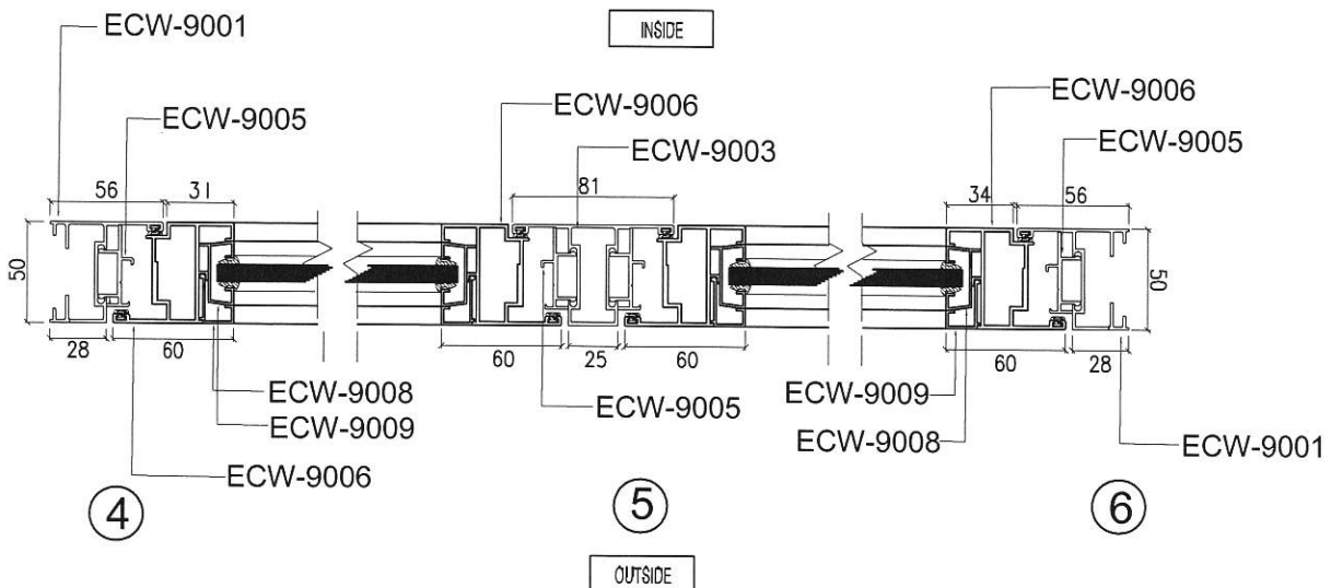
VERTICAL SECTION
