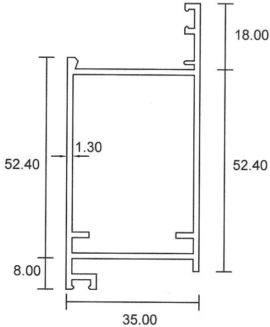
1207 0.807 Kg/m Casement Inner
